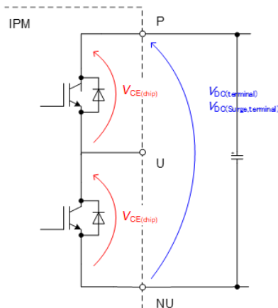
Fig.2-2 Rated Voltage
